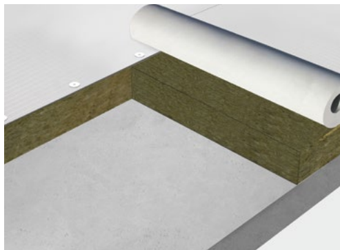
Mechanically fastened installation
